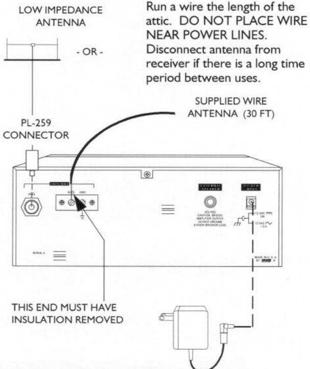
FIGURE 2 - BASIC ANTENNA CONNECTIONS
