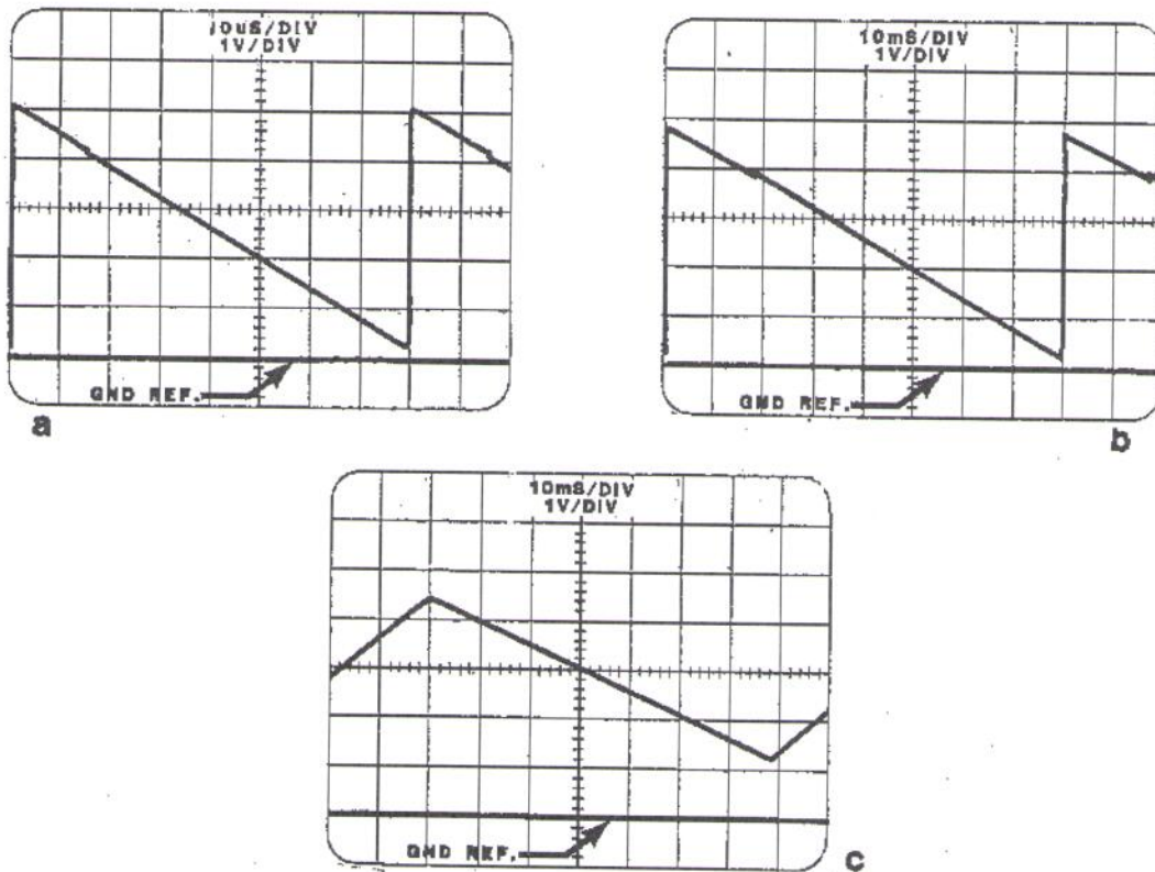
Figure 5-2 Oscilloscope Waveforms
