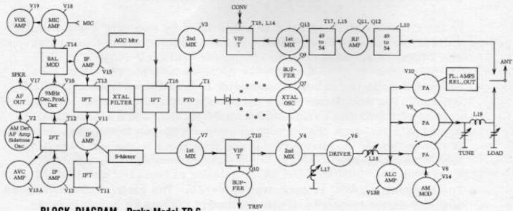
BLOCK DIAGRAM - Drake Model TR-6
