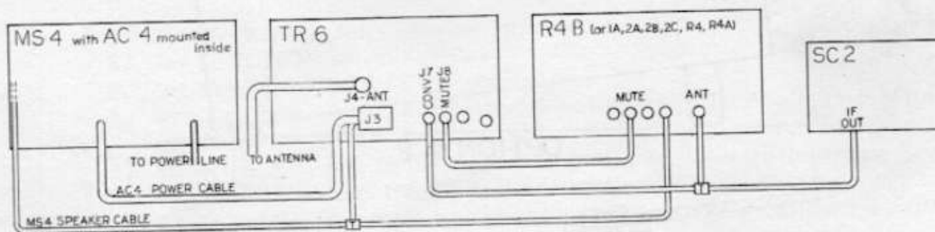
FIG. 7-CONNECTION OF TR 6 WITH AC 4, MS 4, SC 2, AND AN EXTERNAL RECEIVER
