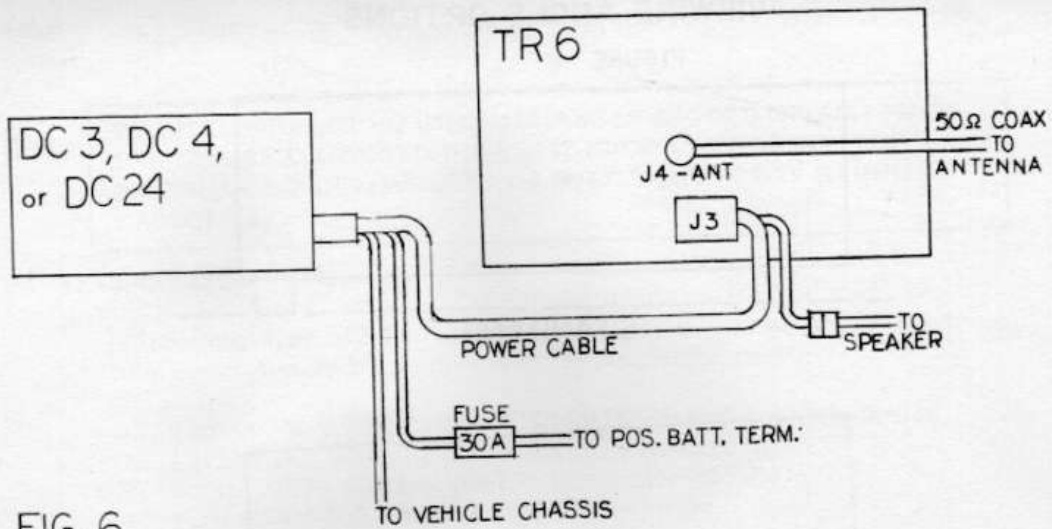
FIG. 6 MOBILE INSTALLATION OF TR 6
