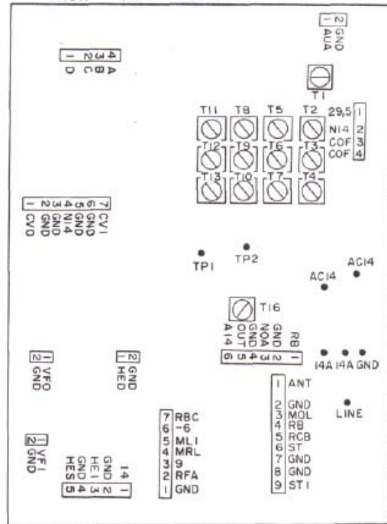
Fig. 38 CONV. Unit
