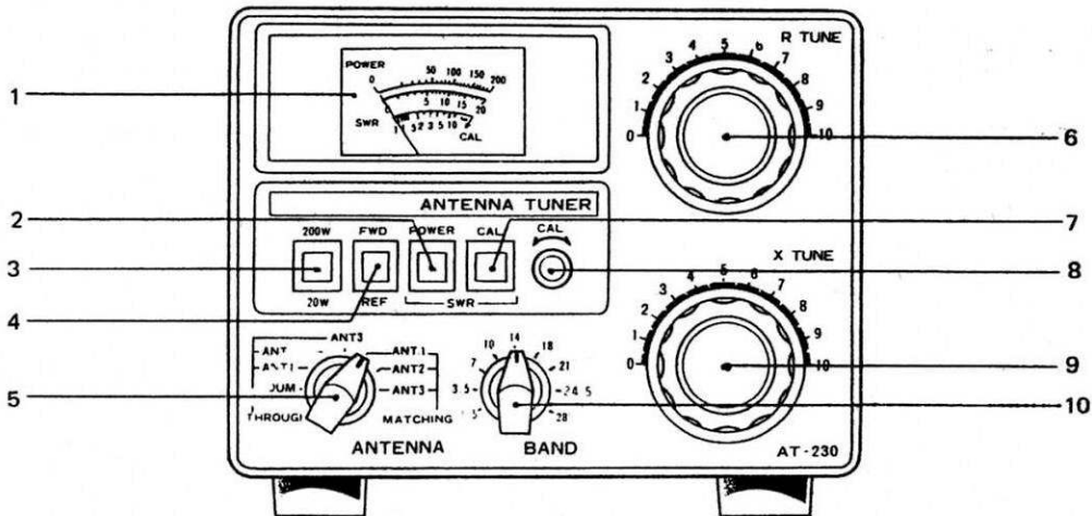
Figure 2-1. Front View
