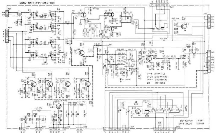
CONV UNIT (X44-1250-00)
