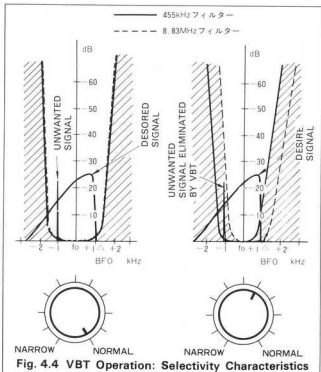
Fig. 4.4 VBT Operation: Selectivity Characteristics
