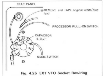
Fig. 4.25 EXT VFO Socket Rewiring
