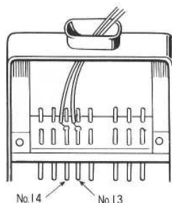
(a) Connections of Socket
