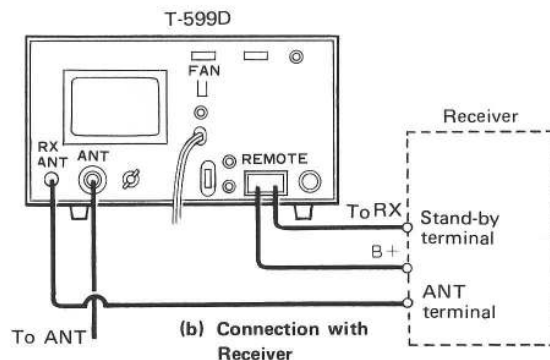
Fig. 17. Connections for a Combination of T-599D and R-599D
