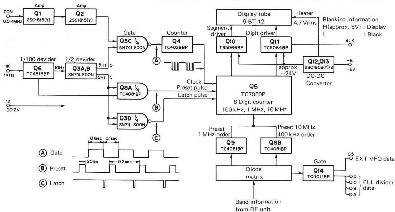
Fig. 3 Counter unit block diagram
