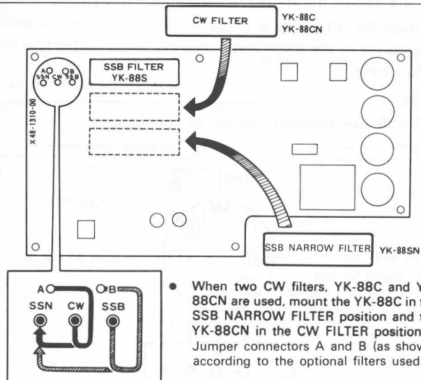
Fig. 5-2 Filter installation
