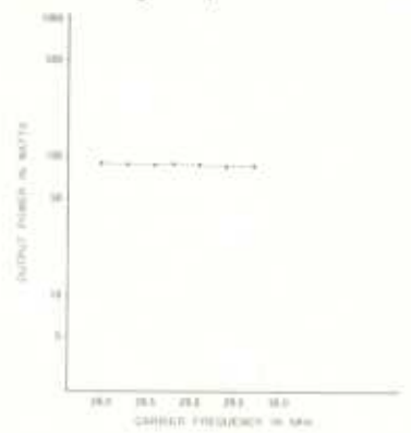
Transmitting output characteristic
