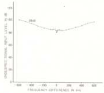
Receiving cross-modulation characteristic
